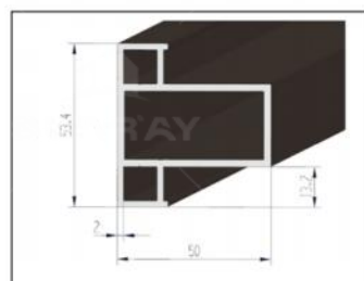
Name : Lower beam frame
