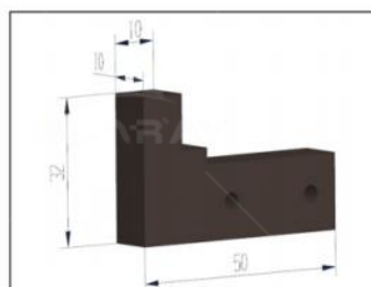
Name : Limit parts
