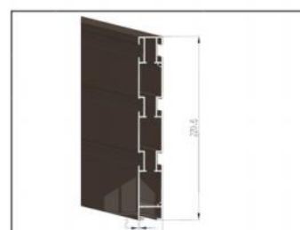
Name: Main beam
