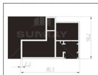
Name: side frame
