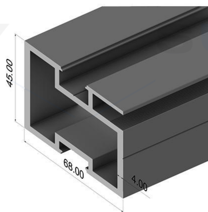
Middle beam
