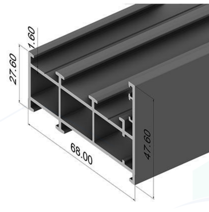
Water retaining rail
