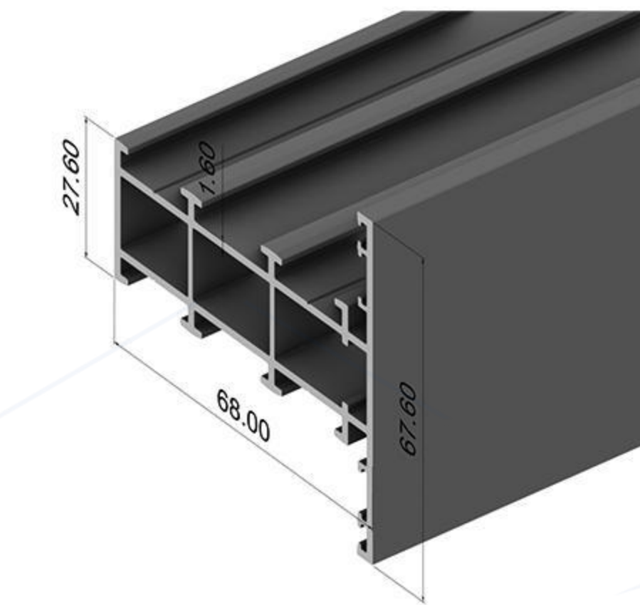
Middle beam
