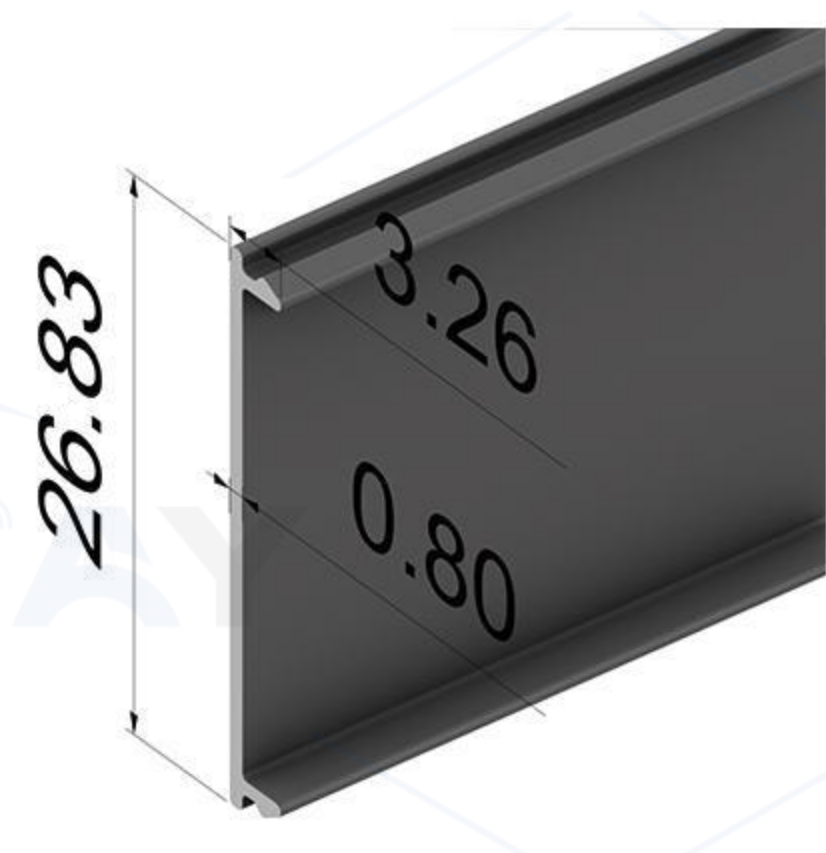
Snap cover
