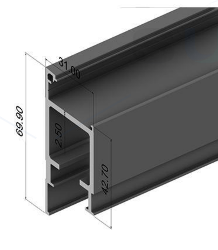
Wall hanging rail
