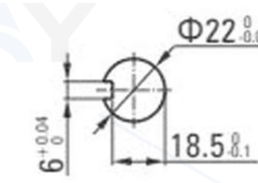
Output shaft structure
