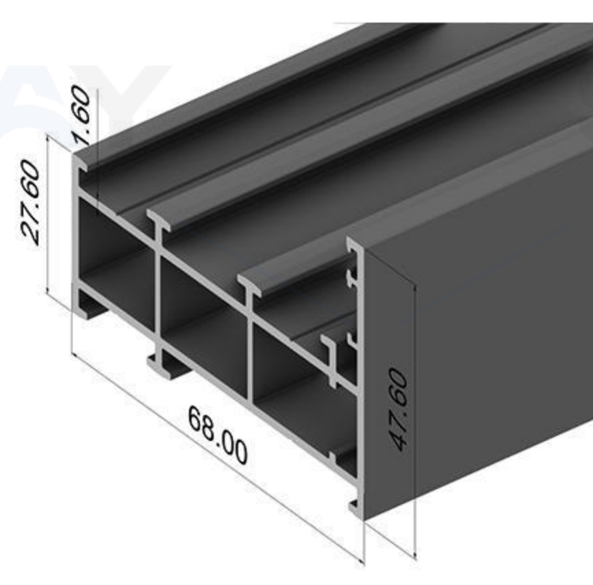
68 frame
