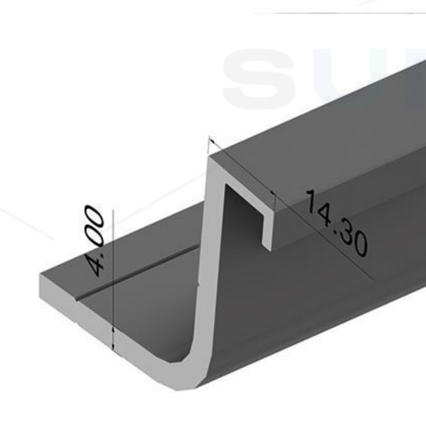
Wall rail plug-in
